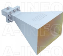
LB-229-15-C-3.5F Standard Gain Horn Antenna 3.3-4.9GHz 15dB Gain 3.5mm Female
