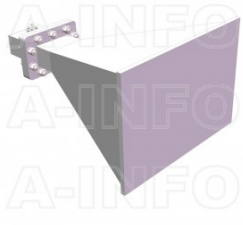
LB-229-15-C-SFSPO Standard Gain Horn Antenna 3.3-4.9GHz 15dB Gain SMA Female
