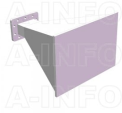
LB-229-15-ASPO Standard Gain Horn Antenna 3.3-4.9GHz 15dB Gain Rectangular Waveguide Interface
